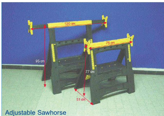
Adjustable Sawhorse
